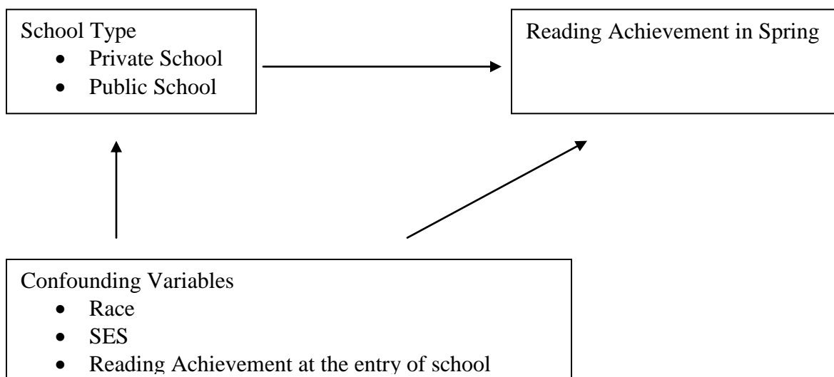
Figure 1: The Model
