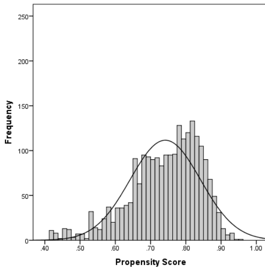
Figure 3: Private School
