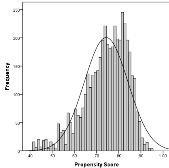
Figure 4: Public School
